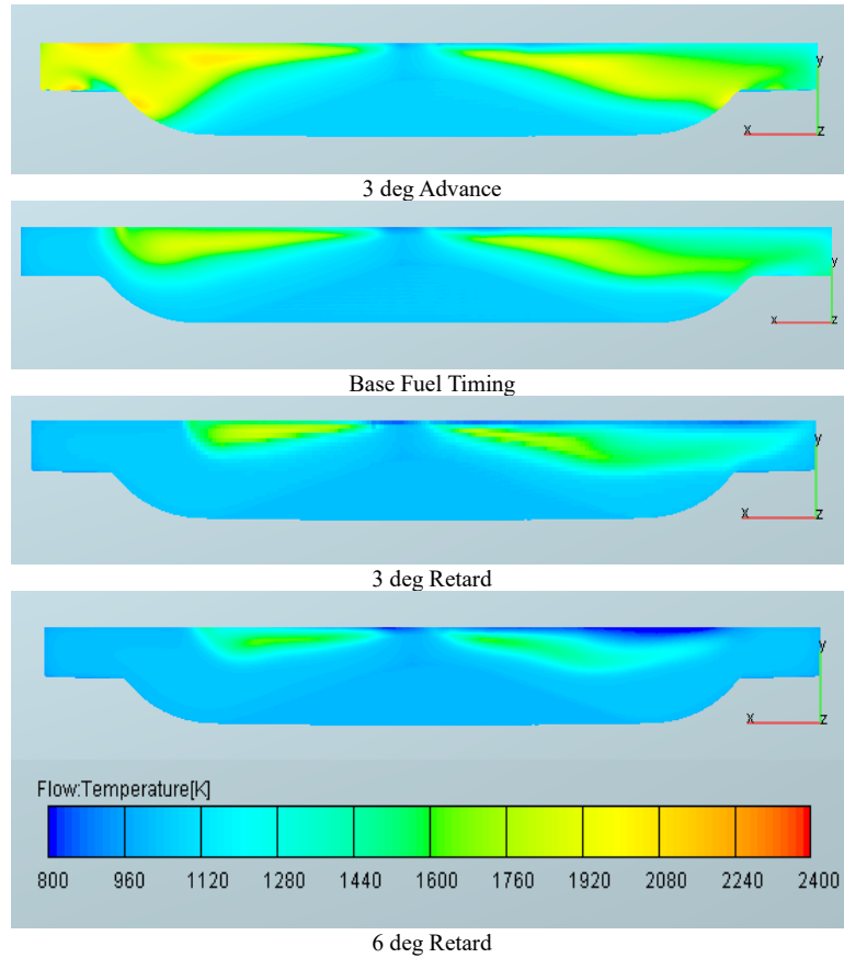
Figure 4. Temperature distribution under different fuel injection conditions at top dead center
