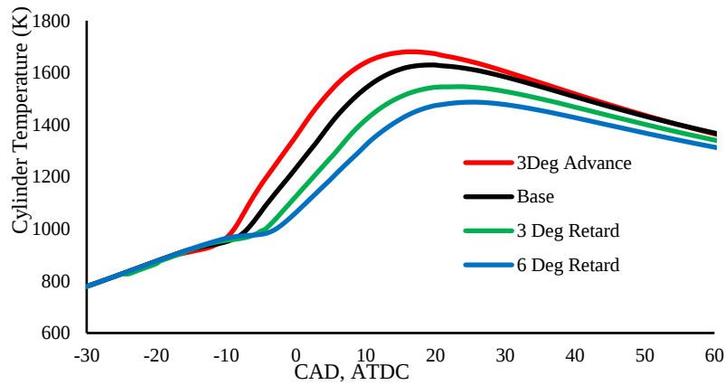
Figure 3. Mean in-cylinder temperature profiles versus crank angle under different fuel injection timing conditions.
