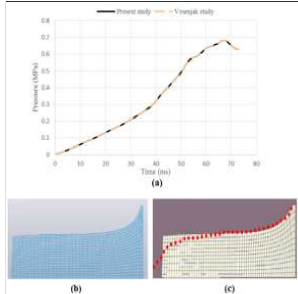
Figure 6. (a) The time variation of water pressure [21]; The free surface of the water under 30g seismic excitation at the time 30 ms: (b) the result of the made model in this study, and (c) Vesenjaj article result [21]
